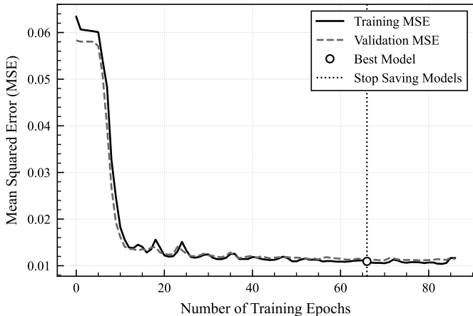
Learning Curve of MHSA-Transformer Model for SolarPlant-1 (Gyeongju)
